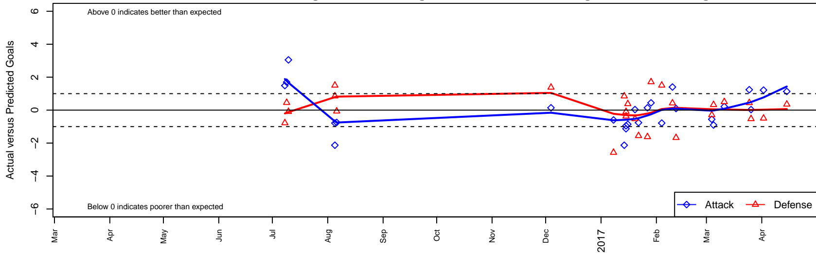
GS Surf A G02 Dots are actual minus expected GF (blue circles) and GA (red triangles). Blue line is smoothed change in attack strength. Red is smoothed change in defense strength.
